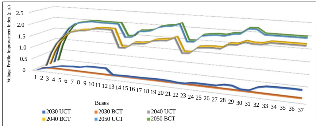
Figure 8. Phase A voltage profile improvement index (VPPI) of the entire network. UCT- undirectional charging technology; BCT- bidirectional charging technology
