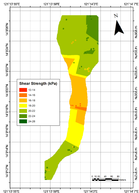
Figure 11. Shear strength map of the recreational area of Makiling Botanic Gardens.
