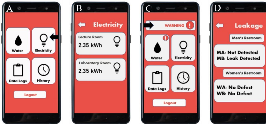
Figure 13. Graphical user interface screenshots of the mobile application's (A) electricity monitoring menu, (B) real-time electricity consumption data, (C) warning notification on water leakage, and (D) detected water leakage location or room.
