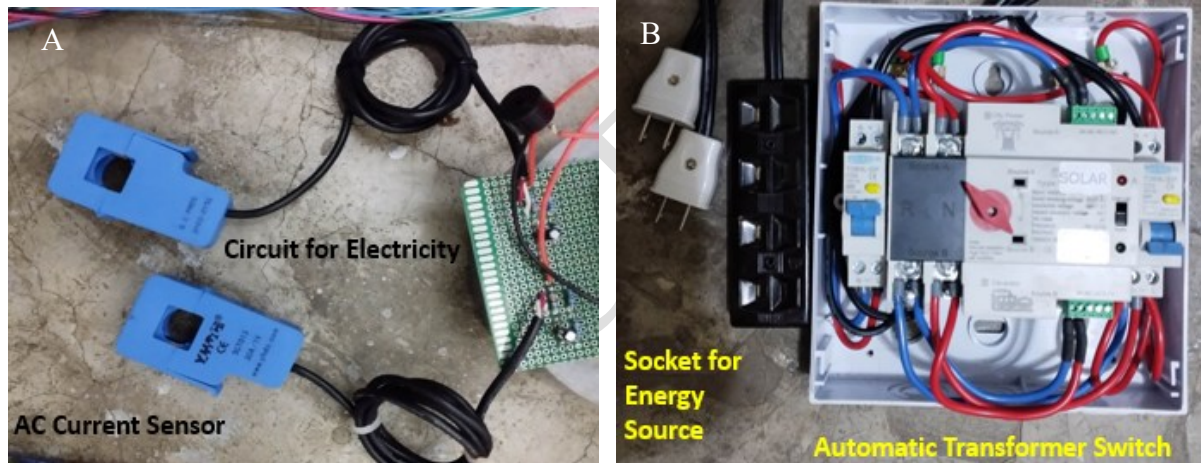
Figure 10. Actual picture of the (A) non-invasive current sensors, and (B) automatic transfer switch
