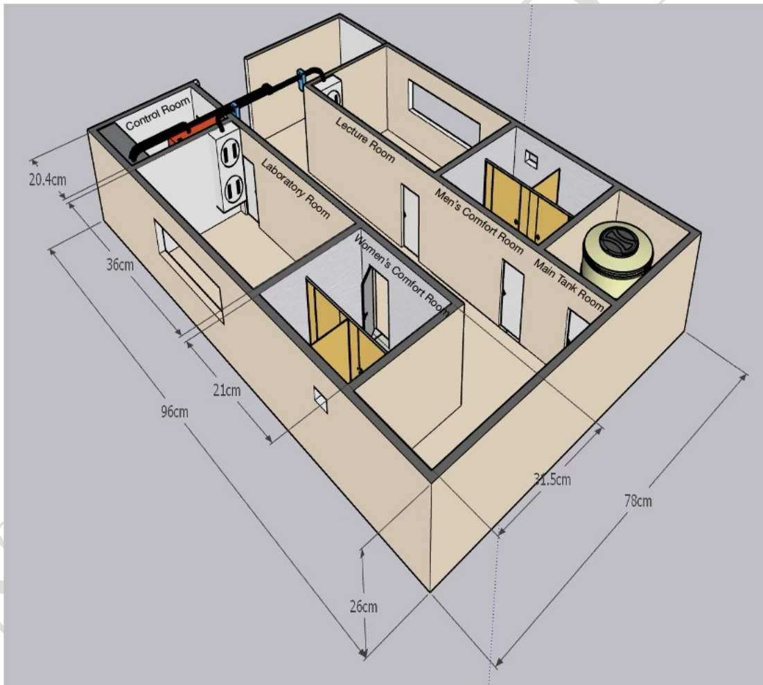
Figure 4. Isometric view of the miniature model showing the dimensions and different rooms.
