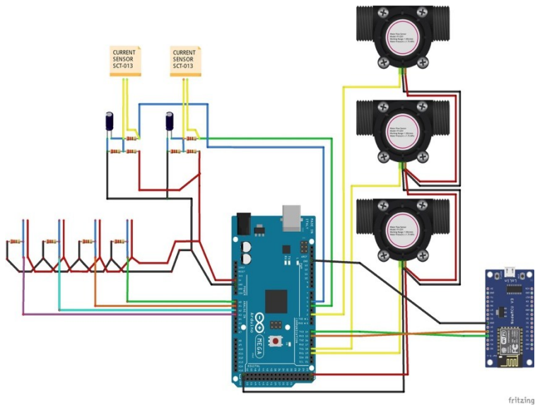
Figure 3. The system's component diagram showing the interface of the input and output modules.
