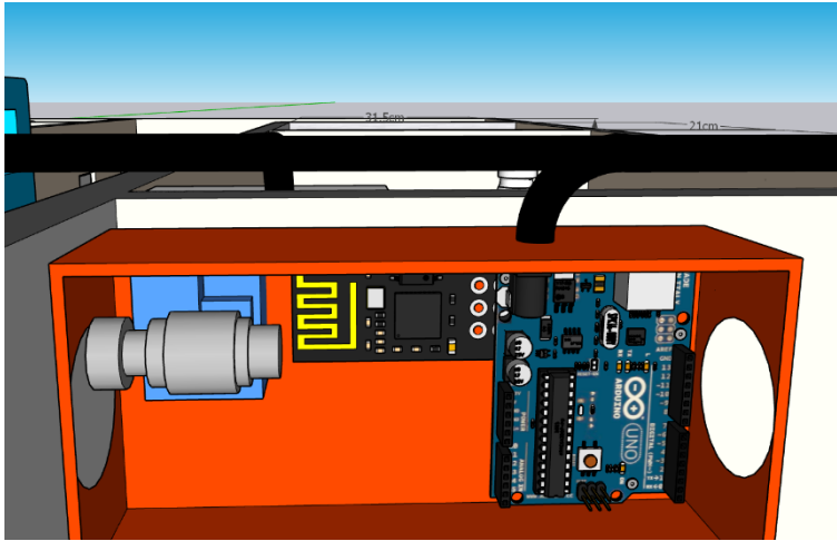
Figure 7. Control room view of the prototype.
