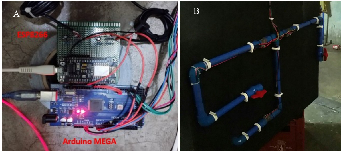
Figure 9. Actual pictures of the (A) ESP8266 WiFi module and Arduino Mega microcontroller, and (B) water flow sensors embedded in the pipelines.
