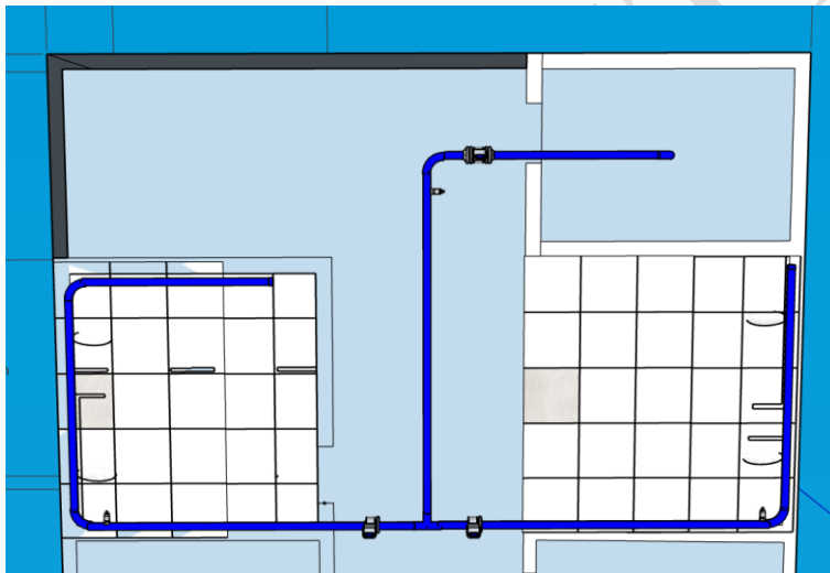
129 Figure 6. Bottom view of the miniature model showing the interconnection of water pipelines.
